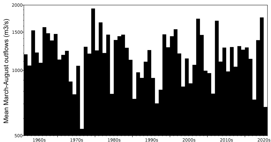
FIGURE 63 | Mean outflows from England for the six-month period March to August from 1961 to 2025 in \text{m}^3/\text{s} . The y-axis is on a logarithmic scale to emphasize the lower outflows.
