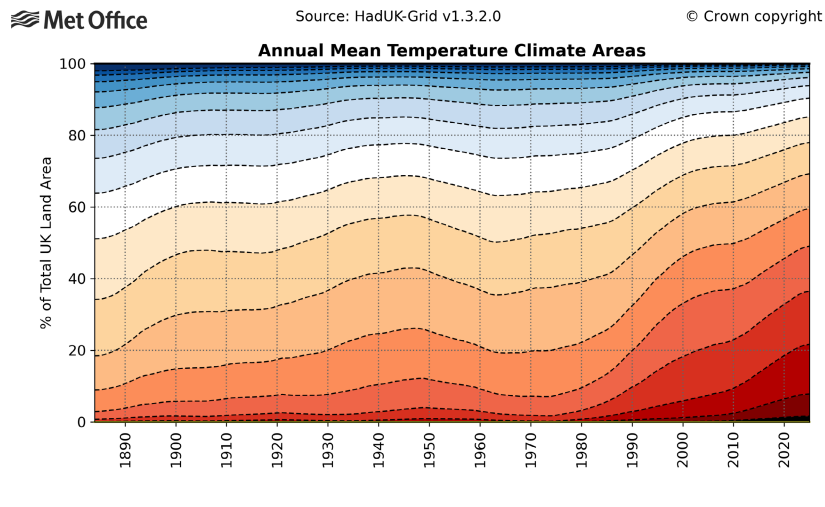
FIGURE 6 | The percentage of total UK land area within 0.5°C intervals of annual mean temperature across the UK from 1884 to 2025. The data have been smoothed to remove the annual variability using a weighted kernel filter described in Appendix A.2.1. The colour scheme is the same as Figure 5.
