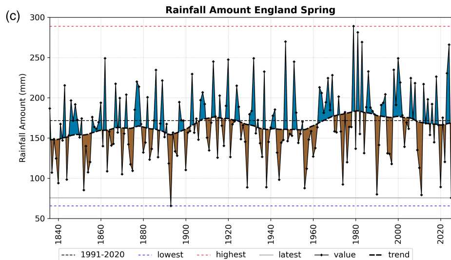
FIGURE 54 | (a) UK mean Tmax (°C) for spring 1884 to 2025, (b) UK sunshine duration (hours) for spring 1910 to 2025 (c) England rainfall (mm) for spring 1836 to 2025.
