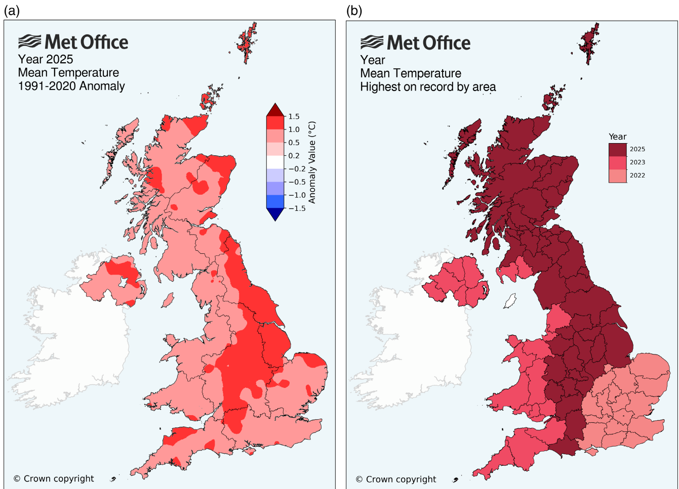
FIGURE 2 | (a) Mean temperature anomaly relative to 1991–2020 for year 2025. Maps for individual months and seasons are available at https://www.metoffice.gov.uk/research/climate/maps-and-data/uk-actual-and-anomaly-maps (b) the warmest year on record for mean temperature for county areas of the UK, based on county series from 1884 to 2025. Appendix A.1.7 describes these county areas. The Isle of Man is not included.
