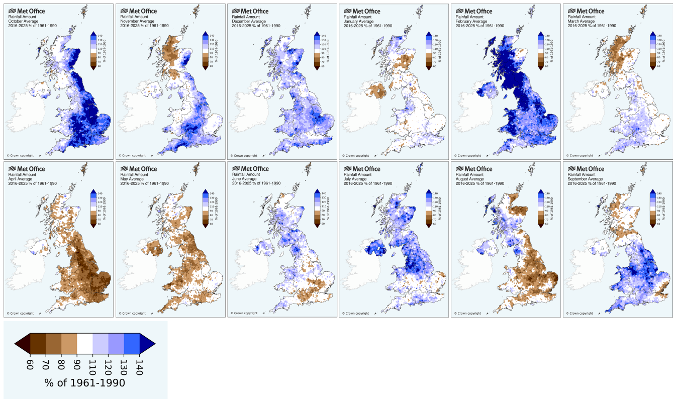
FIGURE 39 | Rainfall anomalies (%) for 2016–2025 for the 12 months of the year: October to March (top) and April to September (bottom) relative to 1961–1990.
