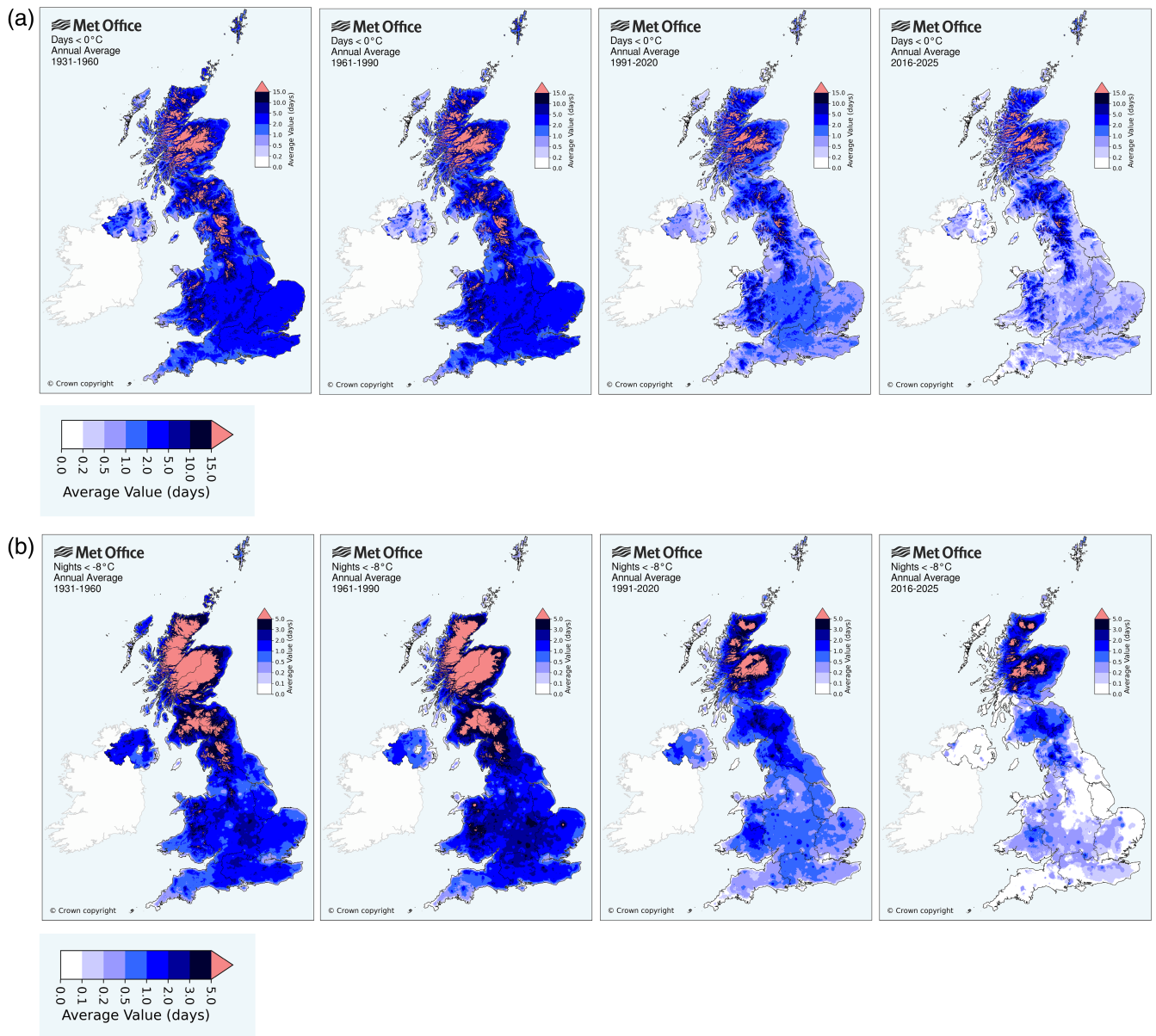
FIGURE 14 | Average number of days per year with (a) daily T_{\max} < 0^{\circ}\text{C} , (b) daily T_{\min} < -8^{\circ}\text{C} for the periods 1931–1960, 1961–1990, 1991–2020 and 2016–2025.
