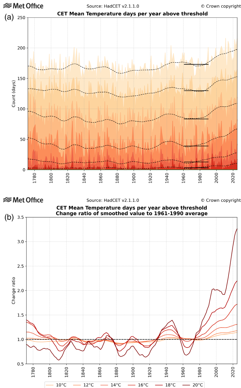
FIGURE 22 | (a) The number of days per year in the daily CET series from 1772 to 2025 with daily Tmean \geq 10^{\circ}\text{C} to 20^{\circ}\text{C} . The hatched lines show the trend (i.e., smoothed) values. The solid black line shows the 1961–1990 average for each series (b) The ‘change ratio’—that is, the ratio of the trend value for each individual year to the 1961–1990 average, for each threshold.
