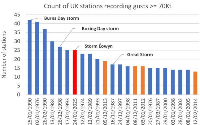
FIGURE 51 | Count of the number of stations recording maximum gust speeds \geq 70 Kt (81 mph) for major UK wind storms in observational records back to 1973. Storm Éowyn is shown in red with other comparatively recent storms 2011, 2012, 2013 and 2014 in orange. Storm dates are listed on the x-axis.
