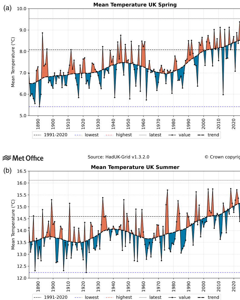
FIGURE 3 | Mean temperature for the UK (°C) from 1884 to 2025 for (a) spring and (b) summer.
