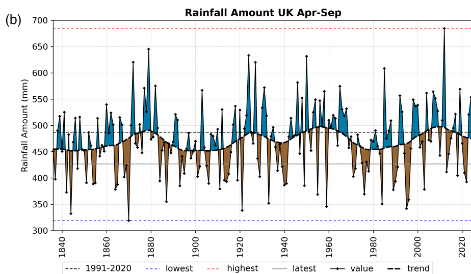
FIGURE 36 | UK half-year rainfall (mm) for (a) October to March 1837 to 2025, (b) April to September 1836 to 2025. The year refers to the month March falls in. The y-axis gridline spacing differs between these figures.
