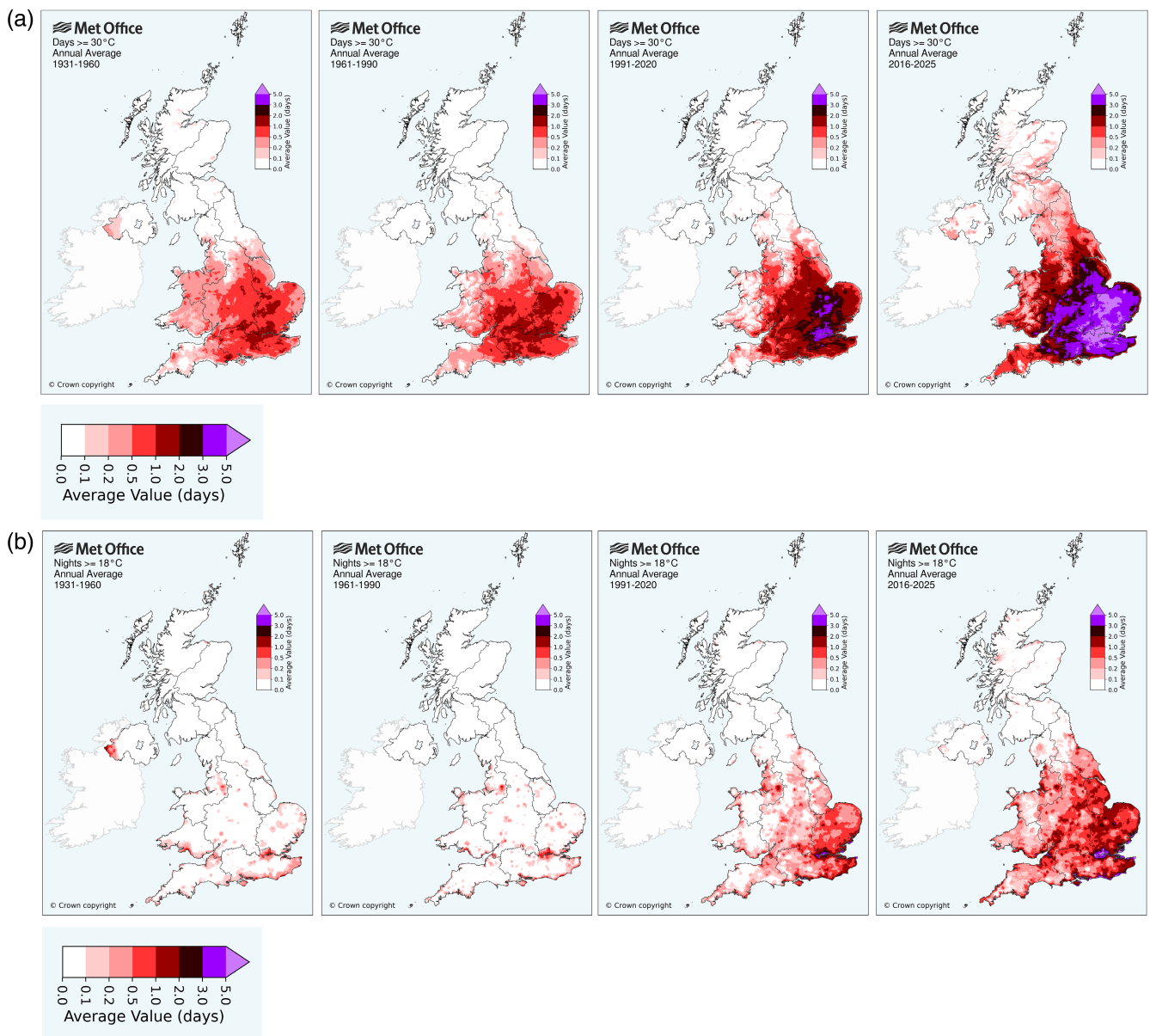
FIGURE 11 | Average number of days per year with (a) daily T_{max} \geq 30^\circ\text{C} , (b) daily T_{min} \geq 18^\circ\text{C} for the periods 1931–1960, 1961–1990, 1991–2020 and 2016–2025. The features on these maps in the west of Northern Ireland relate to a problem with the dataset in this area and should be discounted.
