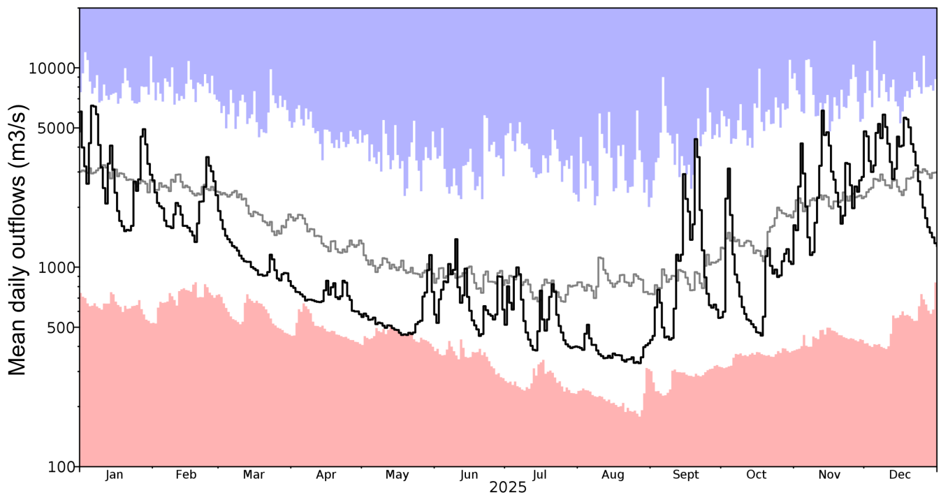
FIGURE 62 | Daily mean outflows from England in 2025 in \text{m}^3/\text{s} (black line). The grey line shows daily long-term average outflows relative to the 1991–2020 standard period, with blue and red the highest and lowest daily outflows on record in the series from 1961. The y-axis is on a logarithmic scale to emphasize the lower outflows.
